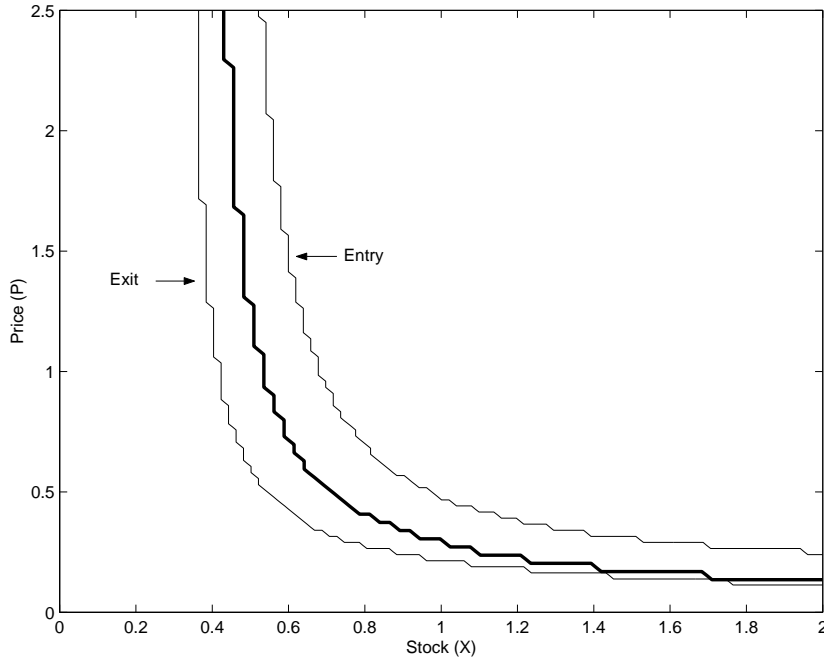
Figure 2: Approximate Switching Curves. Base case (thin lines) and with No switching costs (thick line).
