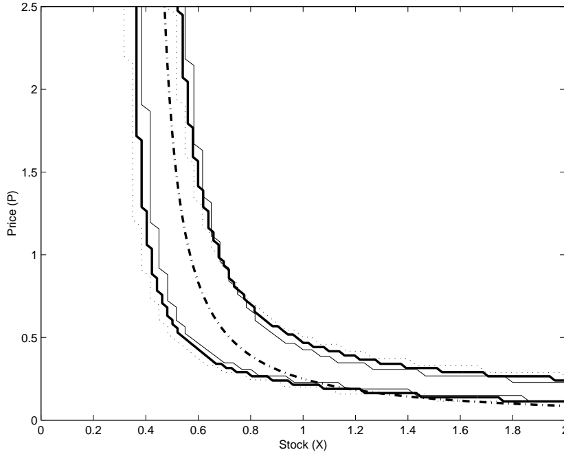
Figure 5: Approximate Switching Curves. Base Case (thick lines), Deterministic (thick dash-dot line), High Volatility with \sigma_X = 0.45 and \sigma_P = 0.30 (thin dashed lines), and Low Volatility with \sigma_X = 0.15 and \sigma_P = 0.10 (thin lines).
