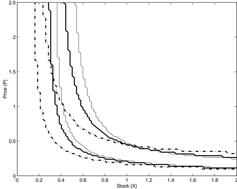
Figure 7: Approximate Switching Curves. Base case (thin lines), Y_{\max} = 0.15 (thick line), and Y_{\max} = 0.05 (thick dash-dot lines).
