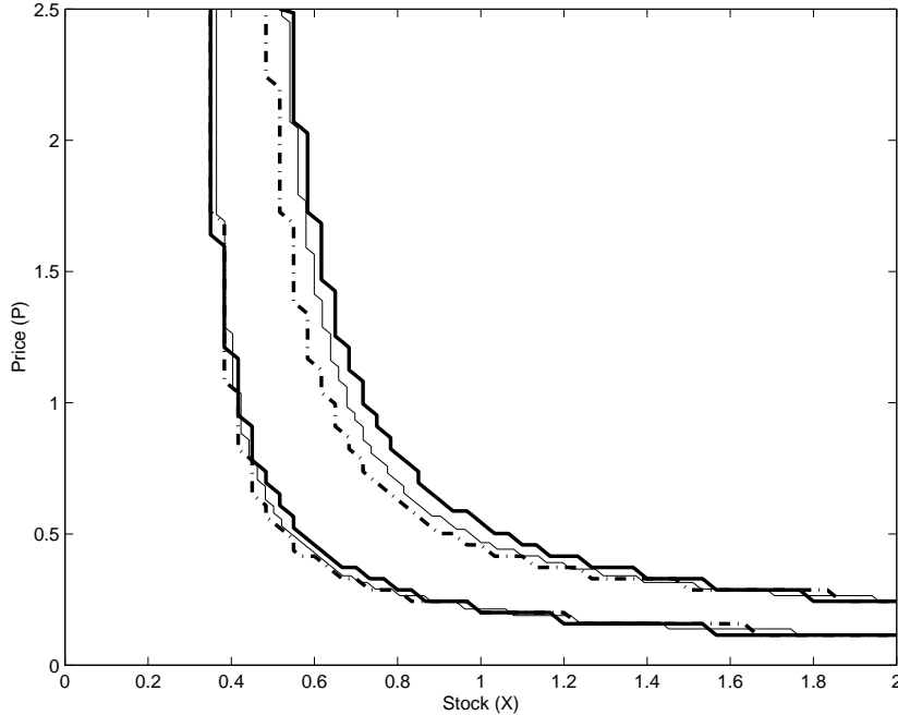
Figure 6: Approximate Switching Curves. Base case r = 0.5 (thin lines), r = 0.25 (thick line), and r = 0.75 (thick dash-dot lines).
